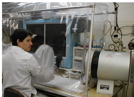
Fig. 7-2. A Coy Laboratory Products (Ann Arbor, MI) anaerobic glove box that is equipped with a catalyst system that uses hydrogen to remove oxygen (courtesy of H.C. Mantovani).
