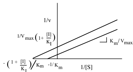
Uncompetitive Inhibition
