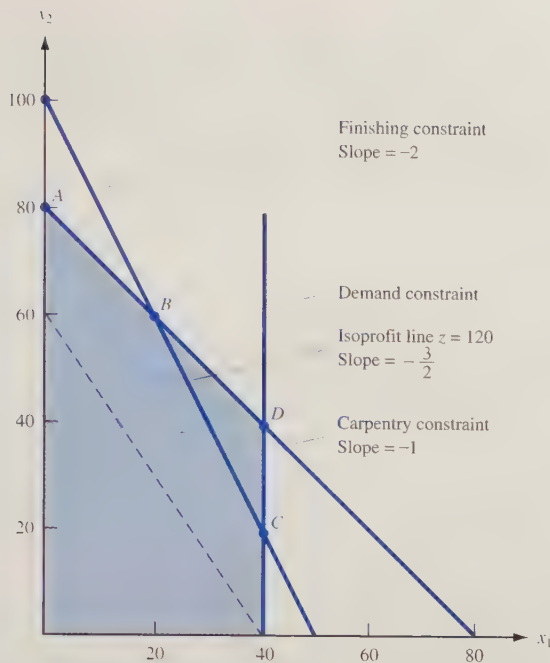
FIGURE 1 Analysis of Range of Values for Which c_1 Remains Optimal in Giapetto Problem
