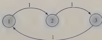
FIGURE 7 A Periodic Markov Chain k = 3
