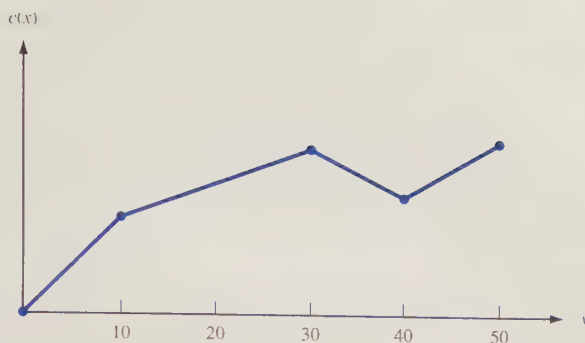
FIGURE 2 A Piecewise Linear Function
