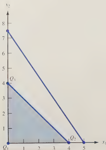
FIGURE 4 Feasible Region for Constraint Set 2
