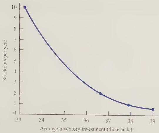
FIGURE 10 Exchange Curve for All and SY
