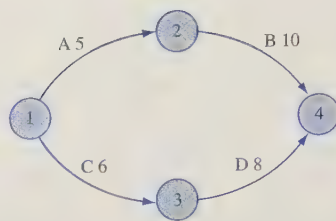
FIGURE 38 Network to Determine Critical Path If Each Activity's Duration Equals m
