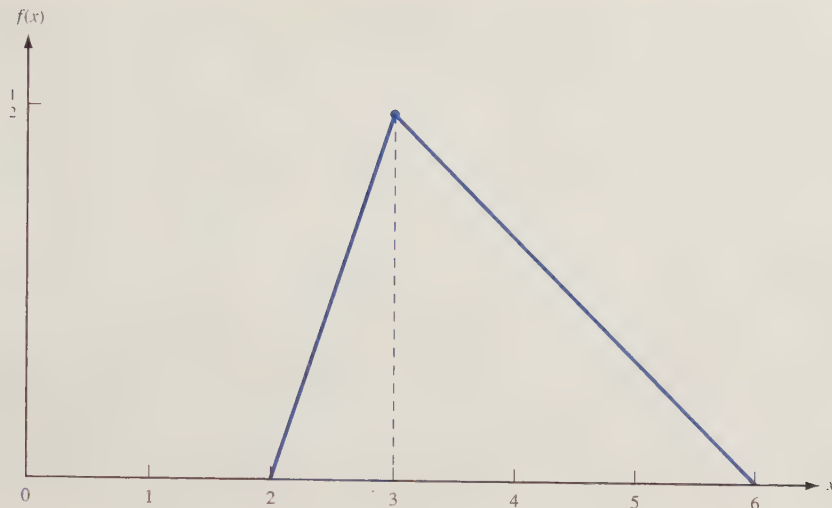
FIGURE 9 Density Function for a Triangular Distribution
