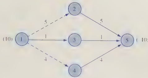
FIGURE 53 Example of a bfs for an MCNFP
