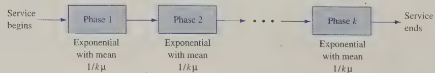
FIGURE 6 Representation of Erlang Service Time
