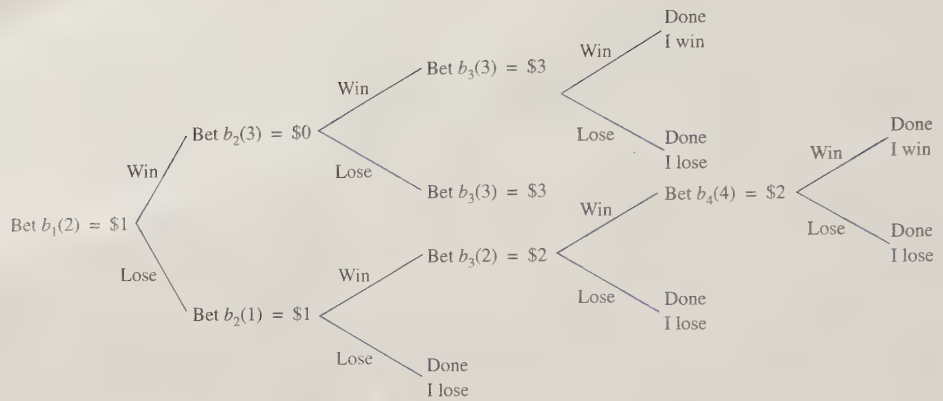
FIGURE 1 Ways Gambler Can Reach $6
