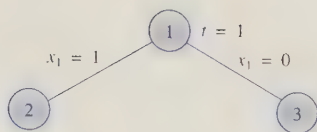
FIGURE 27 Branching on Node 1
