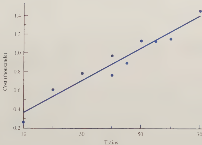
FIGURE 9 Scatterplot of Cost of Producing Trains
