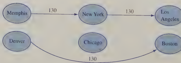
FIGURE 10 Optimal Solution to Widgetco
