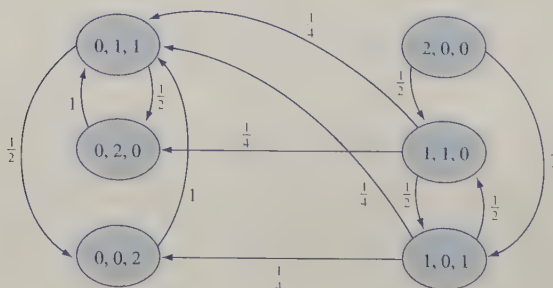
FIGURE 2 Graphical Representation of Transition Matrix for Urn
