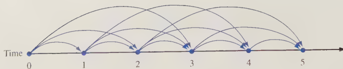
FIGURE 9 Network Representation of Equipment Replacement
