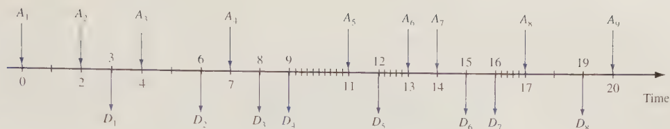
FIGURE 5 Time Continuum Representation of Single-Server Simulation
