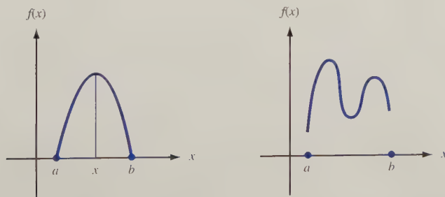
b A function that is not unimodal on [a, b]
