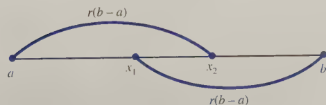
FIGURE 36 Location of x_1 and x_2 for Golden Section Search
