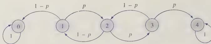
FIGURE 1 Graphical Representation of Transition Matrix for Gambler's Ruin
