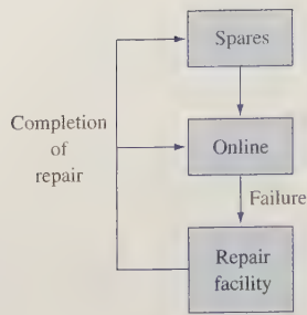
FIGURE 14 Flow of Terminals
