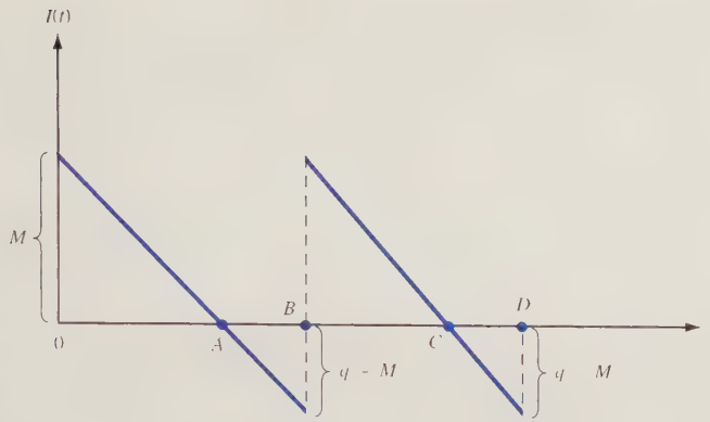
FIGURE 12 Evolution of Inventory over Time for EOQ Model with Back Orders Allowed
