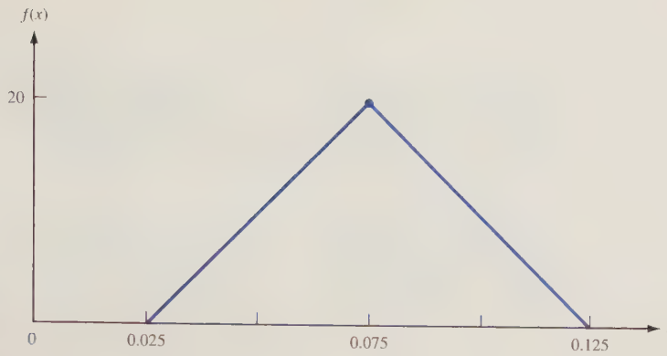
FIGURE 15 The pdf of the Repair Times
