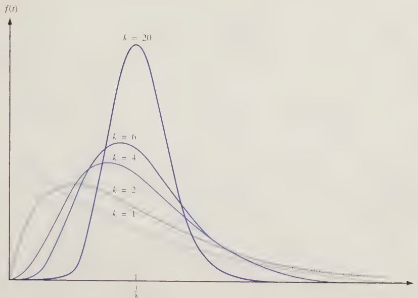
FIGURE 4 Density Functions for Erlang Distributions
