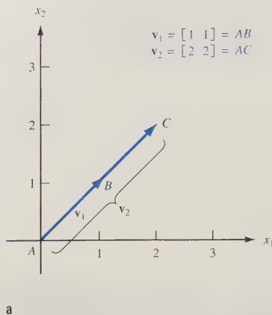
FIGURE 7 (a) Two Linearly Dependent Vectors (b) Two Linearly Independent Vectors
