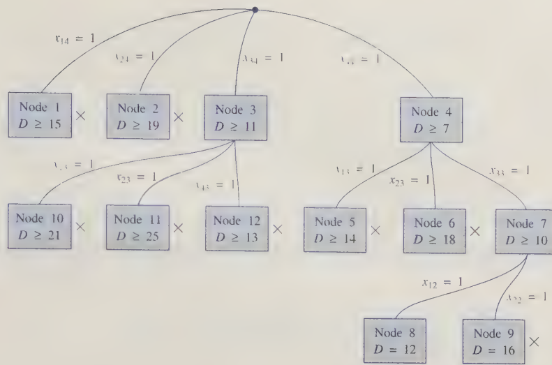
FIGURE 23 Branch-and-Bound Tree for Machine-Scheduling Problem
