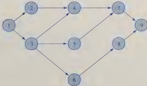
FIGURE 40 Network for Problem 3
