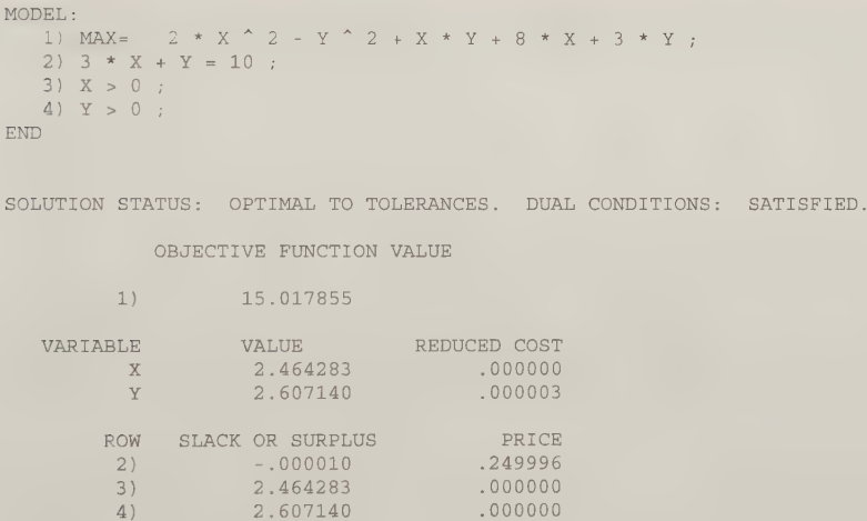
FIGURE 42 Optimal Solution for Example 28
