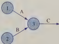
FIGURE 27 Activities A and B Must Be Completed Before Activity C Can Begin
