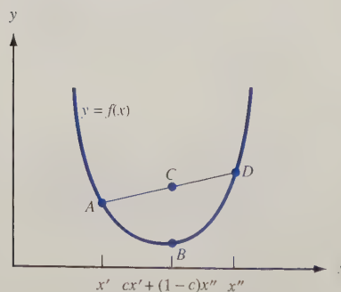
FIGURE 15 A Convex Function
