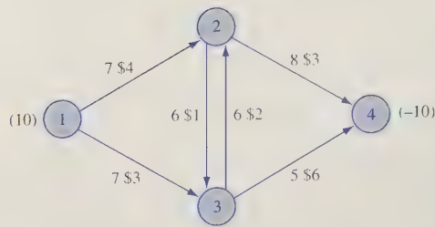
FIGURE 56 Example of Network Simplex
