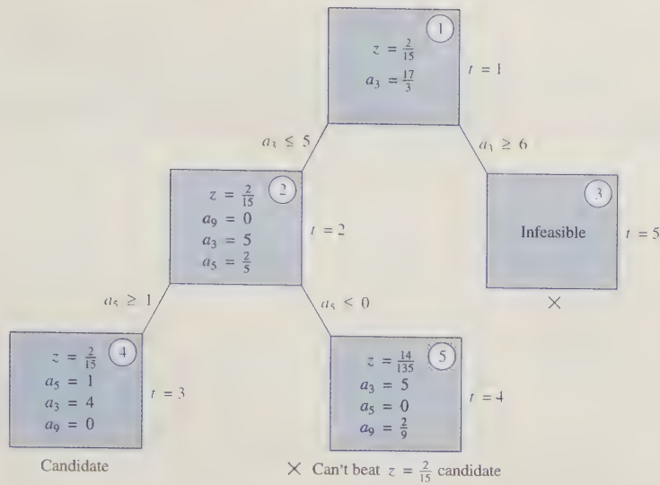
FIGURE 2 Branch-and-Bound Tree for IP (20)
