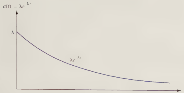
FIGURE 2 Density Function for Exponential Distribution
