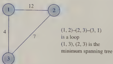
FIGURE 47 Illustration of Loop and Minimum Spanning Tree
