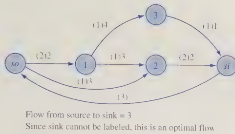
FIGURE 16 Network for Sunco Oil (Optimal Flow)
