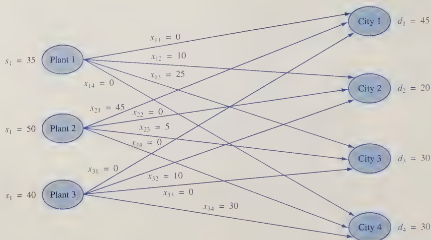
FIGURE 1 Graphical Representation of Powerco Problem and Its Optimal Solution
