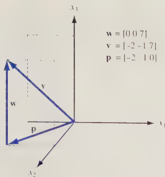
FIGURE 5 Projection of [−2 −1 7] onto x_3 = 0
