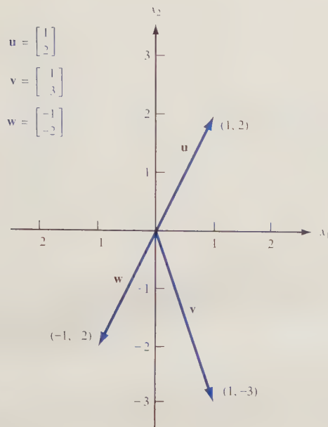
FIGURE 1 Vectors Are Directed Line Segments
