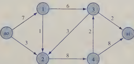
FIGURE 22 Network for Problem 5
