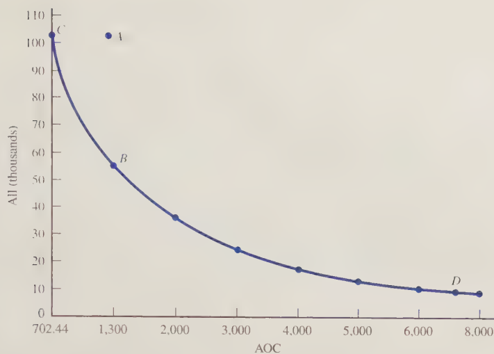
FIGURE 9 Example of an Exchange Curve
