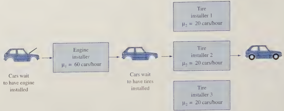
FIGURE 25 Series Queuing System for Automobile
