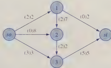
c Label sink by so - 1 - 2 - 3 - si (adds 2 units of flow using only forward arcs)
