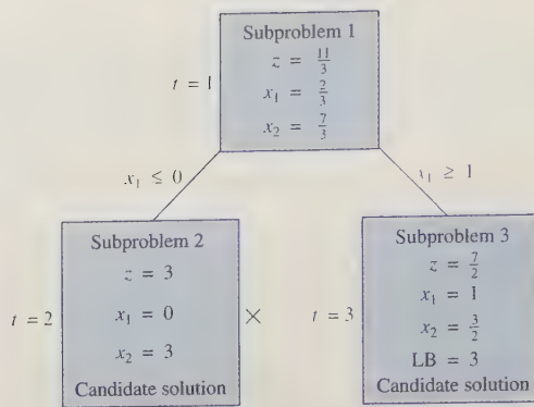
FIGURE 21 Branch-and-Bound Tree for Mixed IP
