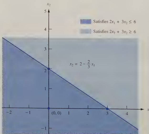
FIGURE 1 Graphing a Linear Inequality
