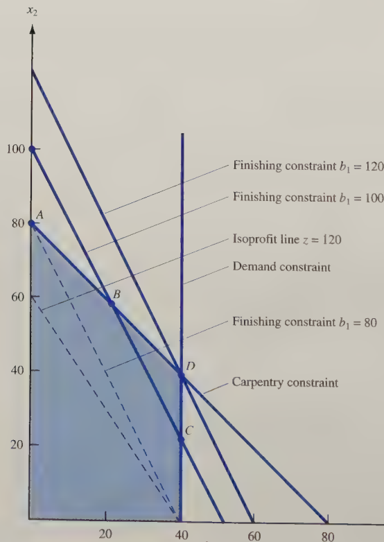
FIGURE 2 Range of Values of Finishing Hours for Which Current Basis Remains Optimal in Giapetto Problem
