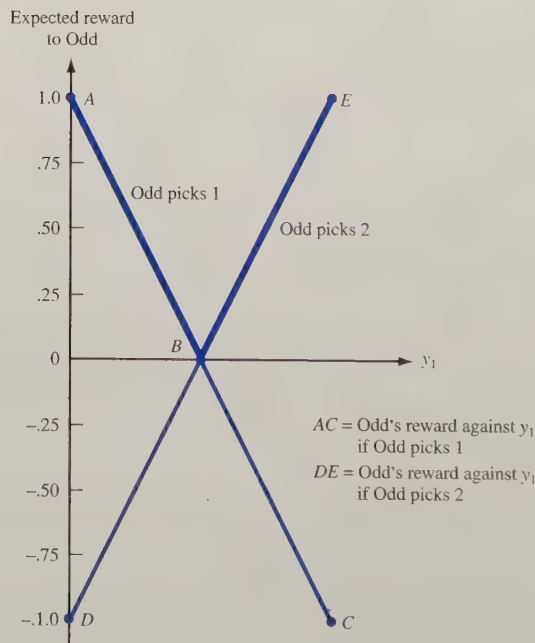
FIGURE 2 Choosing Even's Strategy
