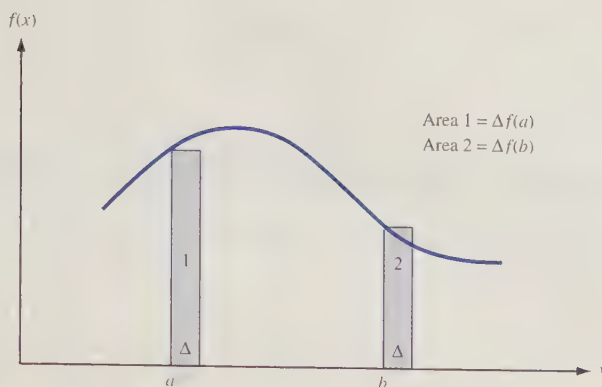
FIGURE 5 Illustration of Probability Density Function
