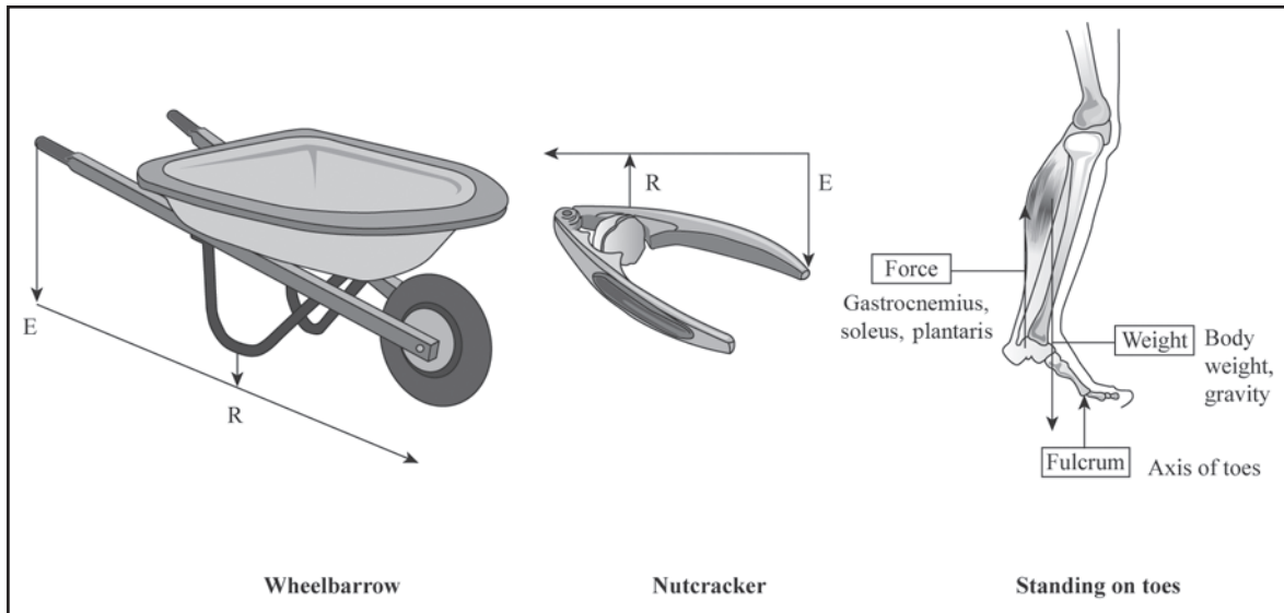
Figure 2-25. Examples of second-class levers.
