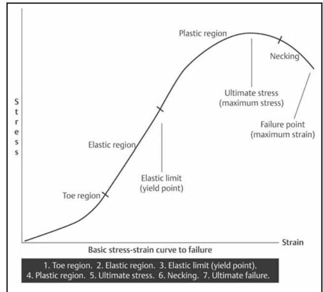
Figure 12-5. Stress-strain curve.
