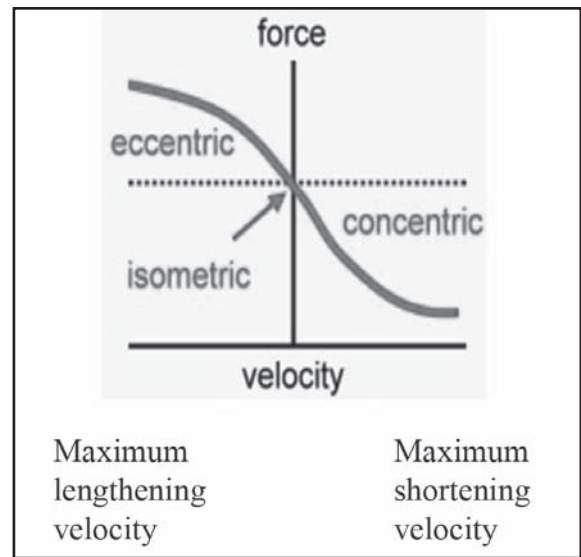
Figure 4-8. Force-velocity curve.
