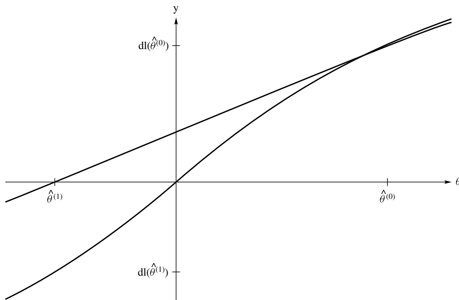
Figure 6.2.1: Beginning with the starting value \hat{\theta}^{(0)} , the one-step estimate is \hat{\theta}^{(1)} , which is the intersection of the tangent line to the curve l'(\theta) at \hat{\theta}^{(0)} and the horizontal axis. In the figure, dl(\theta) = l'(\theta) .
