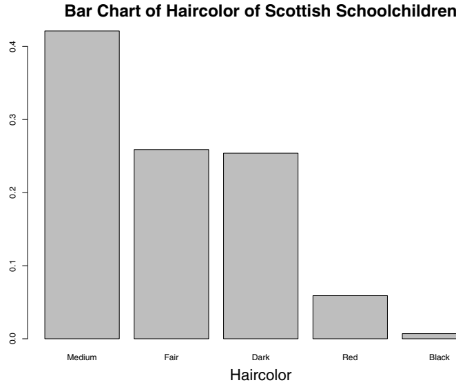
Figure 4.1.1: Bar chart of the Scottish hair color data discussed in Example 4.1.5.
