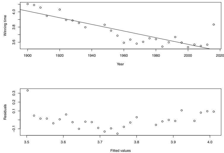
Figure 9.6.2: The top panel is the scatterplot of winning times in the men's 1500 meters versus the year of the Olympics. The least squares fit is overlaid. The bottom panel is the residual plot of the fit.
