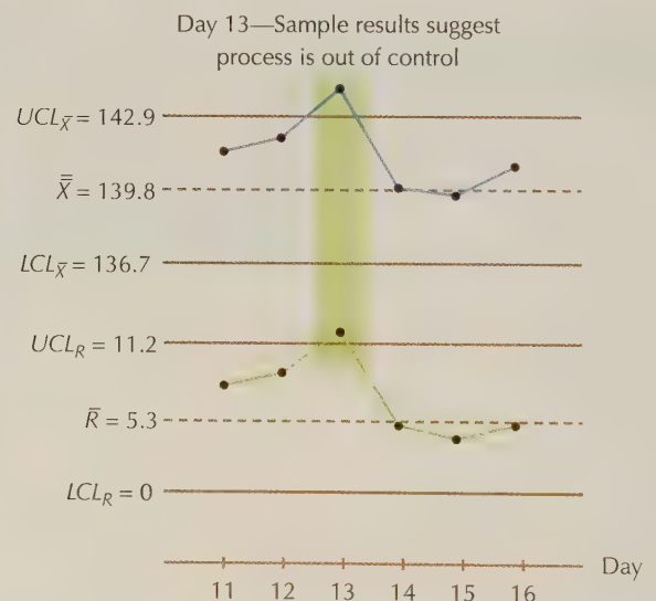
FIGURE 5.8 Control Chart Results for Days 11 through 16
