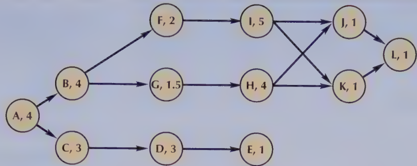
FIGURE 14.10 Network Diagram for the GriddleIron Project
