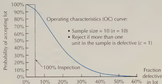
FIGURE 5.9 OC Curve for Chapman Industries
