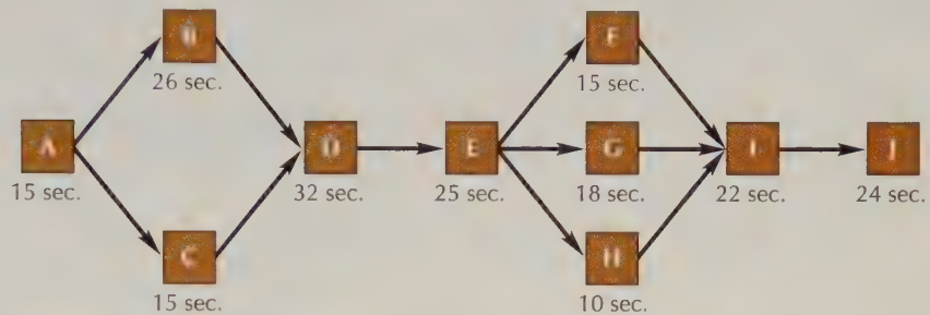
FIGURE 3.15 Precedence Diagram for Blackhurst Engineering
