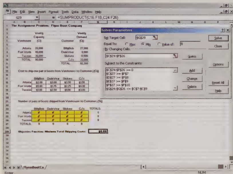
FIGURE 8.10 Solver Dialog Box for Flynn Boot Company Example
